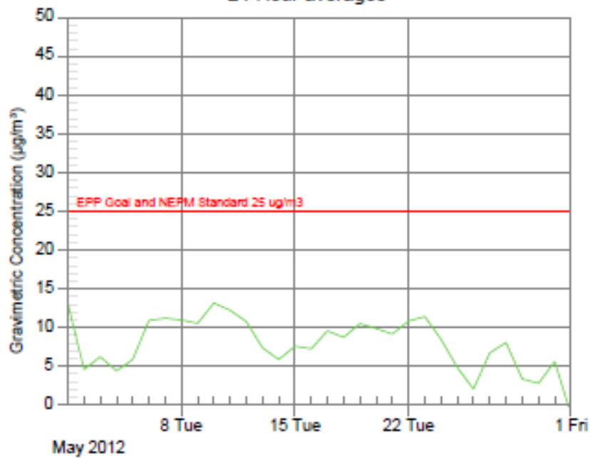
PM 2.5 LandCentre 24 Hour averages
