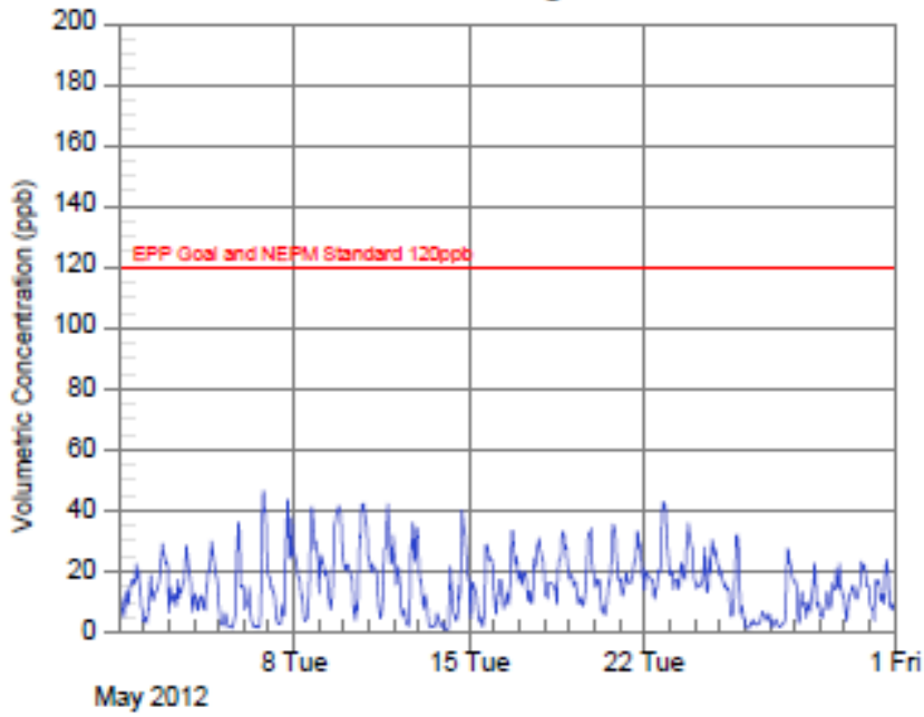
NO 2 Hawthorne St 1 Hour averages
