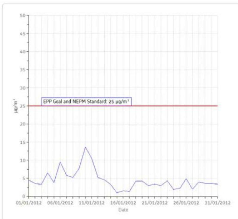
PM 2.5 _MC[µg/m 3 ] Station: RBH Monthly: 01/2012 Type: AVG 1 Day
