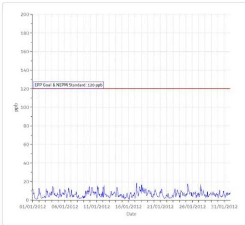
NO 2 [ppb] Station: RBH Monthly: 01/2012 Type: AVG 1 Hr.
