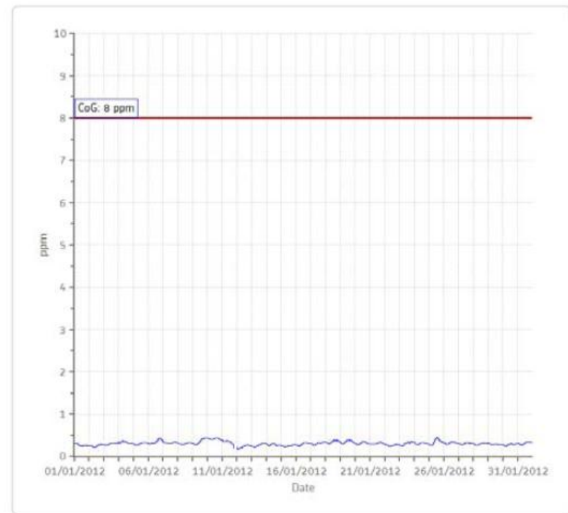
CO[ppm] Station: RBH Monthly: 01/2012 Type: RunningAvg 8 Hrs.
