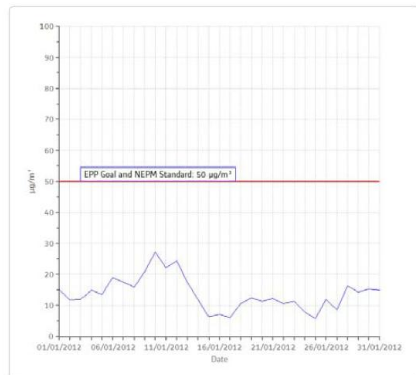
PM 10 [µg/m 3 ] Station: RBH Monthly: 01/2012 Type: AVG 1 Day
