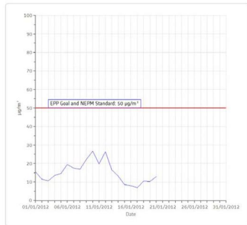
PM 10 [µg/m 3 ] Station: LANDCENTRE Monthly: 01/2012 Type: AVG 1 Day
