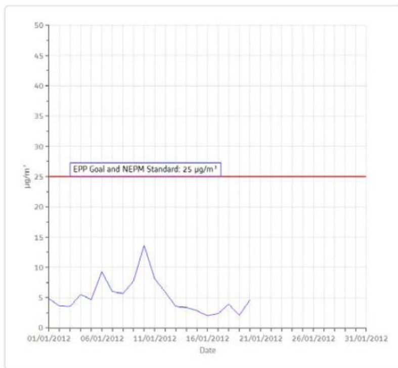
PM 2.5 _MC[µg/m 3 ] Station: LANDCENTRE Monthly: 01/2012 Type: AVG 1 Day
